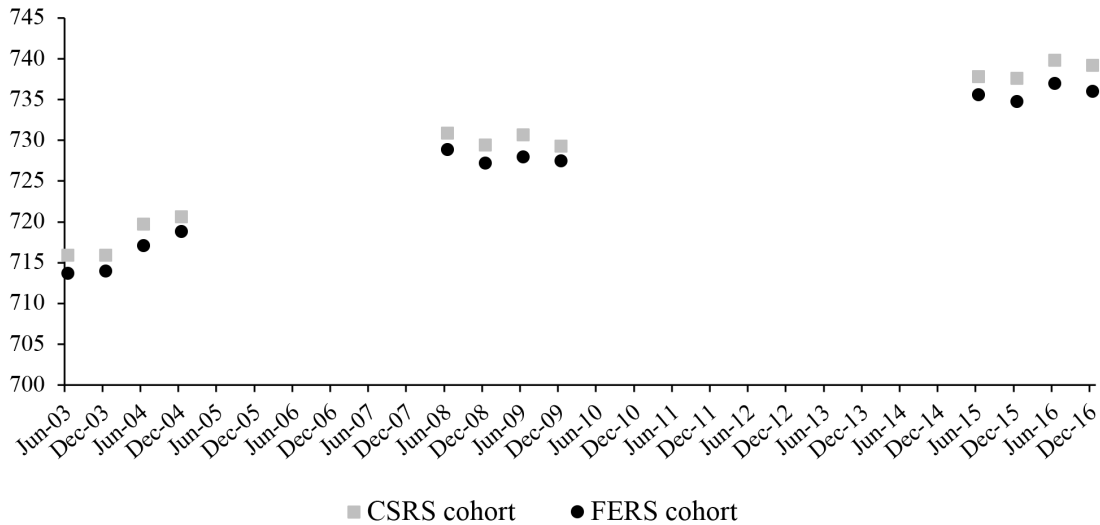
Figure 3. Vantage score
